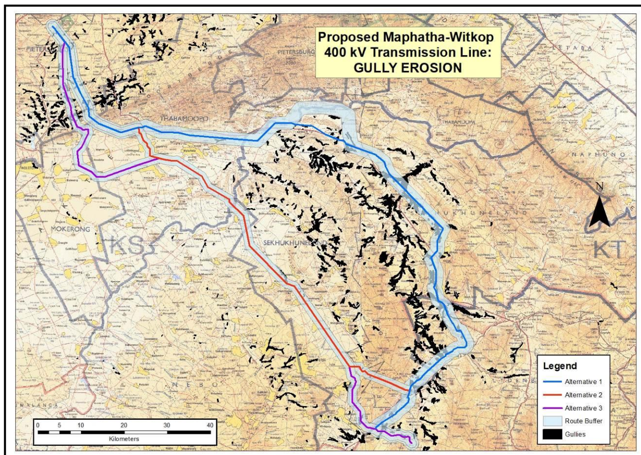
Figure 4. Gully erosion
